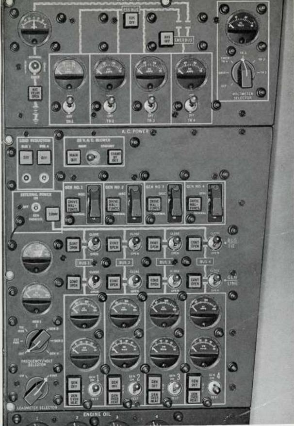
FLIGHT ENGINEER'S PANEL
