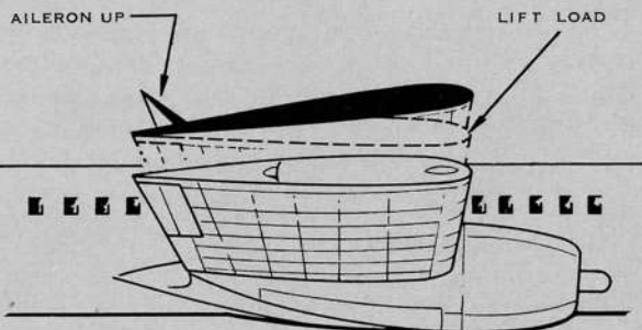
CONTROL REVERSAL — LONG FLEXIBLE WING WITH OUTBOARD AILERON
