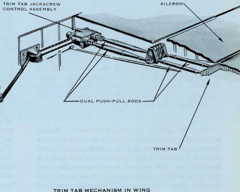
TRIM TAB MECHANISM IN WING
