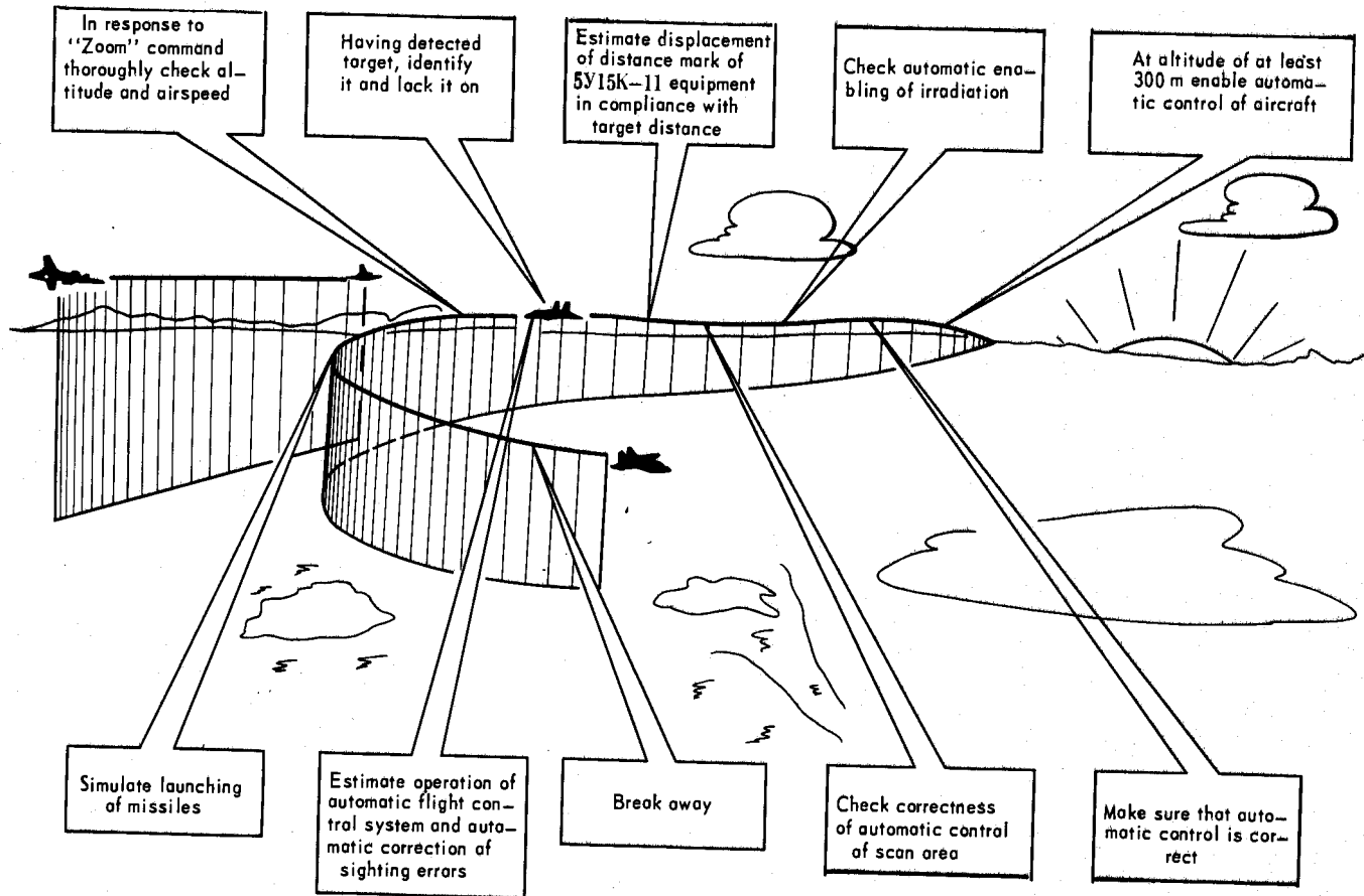
FIG. 148. PATTERN OF FORWARD-CONE ATTACK
