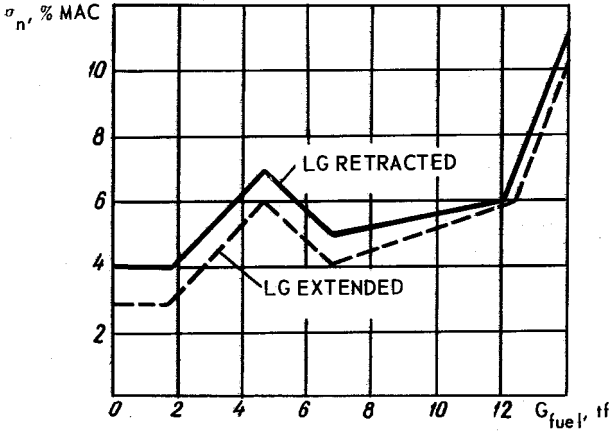
FIG. 21. VARIATION OF AIRCRAFT ANGLE-OF-ATTACK STABILITY MARGIN \sigma_n WITH FUEL UTILIZATION TAKEN INTO ACCOUNT (pitch damper is engaged, aircraft carries four missiles P-40.1, M_{\text{act}} = 0.8 )
