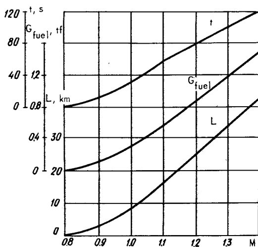
FIG. 14. ACCELERATION CHARACTERISTICS OF AIRCRAFT CARRYING FOUR MISSILES P-40 AT FULL REHEAT POWER SETTING ( H = 8000 m, G = 30 tf)
