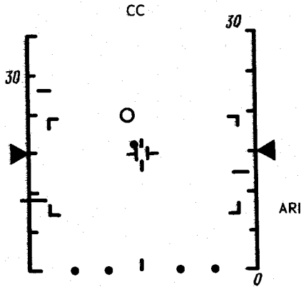
FIG. 139. PICTURE DISPLAYED ON RADAR INDICATOR SCREEN IN AUTOMATIC DIRECTION (mode T- \psi_0 I)
