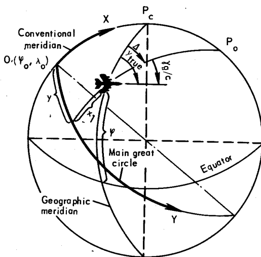
FIG. 45. GREAT-CIRCLE SYSTEM OF COORDINATES
