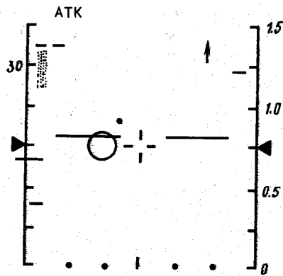
FIG. 129. PICTURE DISPLAYED ON RADAR INDICATOR SCREEN AT HOMING STAGE (rear-cone attack launched against passive jammer, fighter position control, mode MLA)
