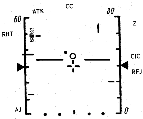
FIG. 121. PICTURE DISPLAYED ON RADAR INDICATOR SCREEN AT HOMING STAGE (attack launched against active noise jammer with missiles P-40P1)
