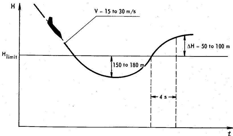
FIG. 35. FLIGHT PATH IN LIMIT ALTITUDE RECOVERY MODE
