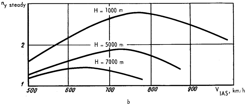
FIG. 41. G-LOAD n_{y \text{ steady}} IN STEADY 360^\circ TURN VERSUS V_{IAS} AND FLIGHT ALTITUDE H
