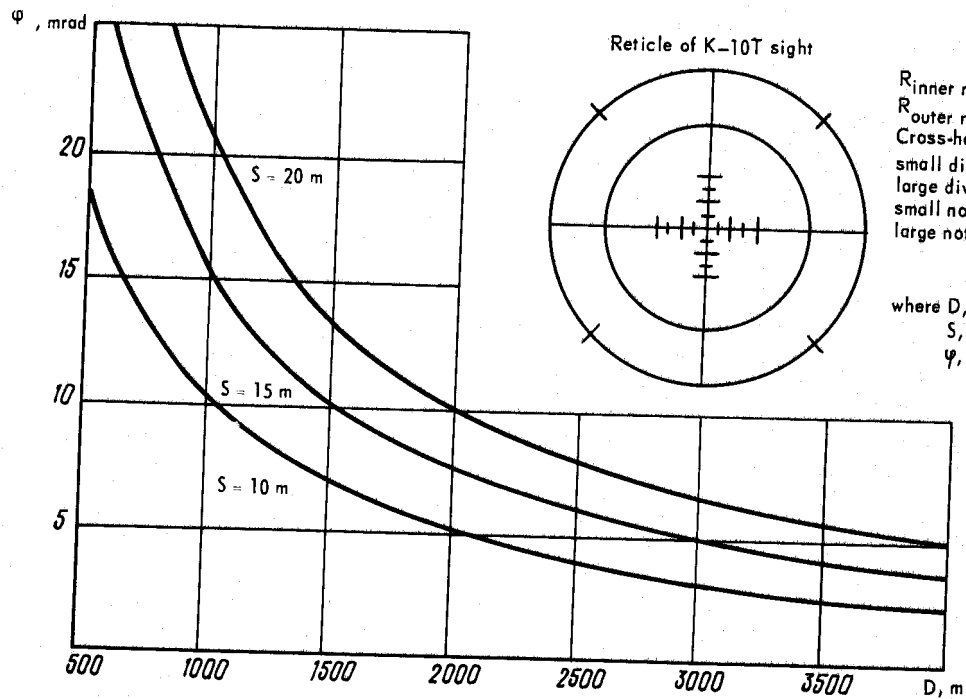
FIG. 147. COLLIMATING SIGHT K-10T
