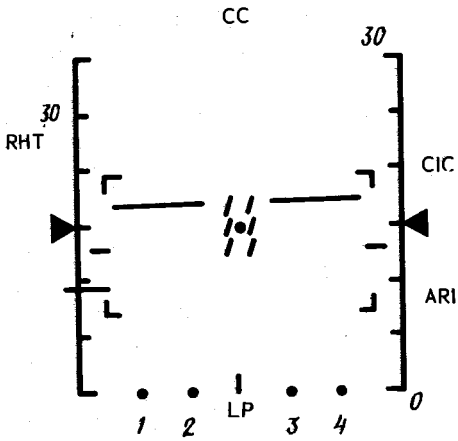
FIG. 140. PICTURE DISPLAYED ON RADAR INDICATOR SCREEN IN AUTOMATIC DIRECTION (mode T- \psi_0 II)
