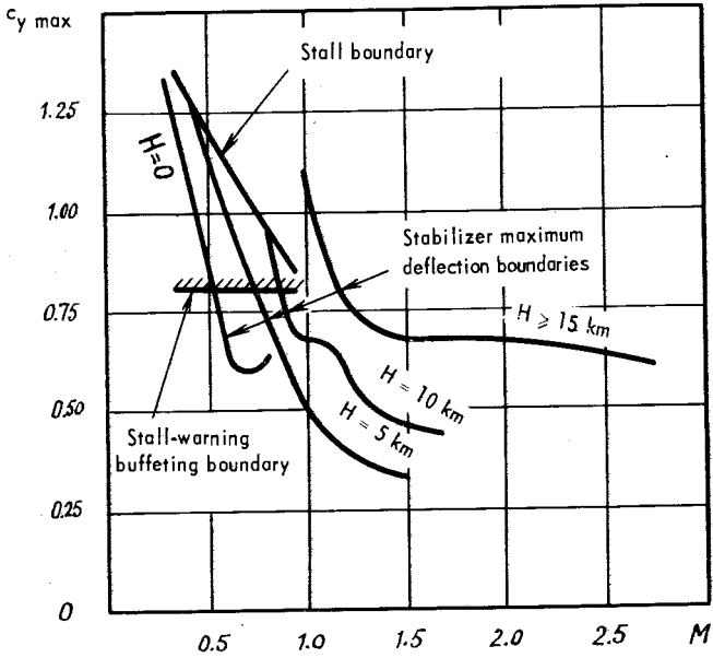
FIG. 9. MAXIMUM LIFT COEFFICIENT c_{y \max} VERSUS MACH NUMBER (aircraft carries four missiles P-40A)
