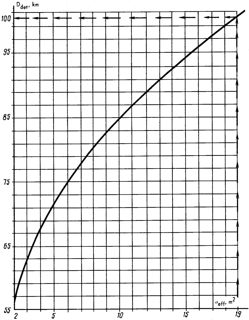
FIG. 98. "SAPFIR-25" AIRBORNE RADAR TARGET DETECTION RANGE VERSUS EFFECTIVE REFLECTING SURFACE OF TARGET ( \sigma = 2 to 19 m^2 )
