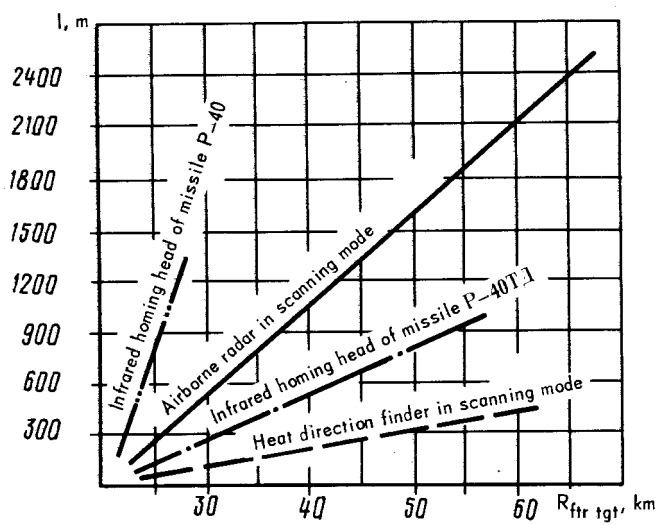
FIG. 159. RESOLUTION OF RADAR, HEAT DIRECTION FINDER AND MISSILES IN AZIMUTH AND ELEVATION
