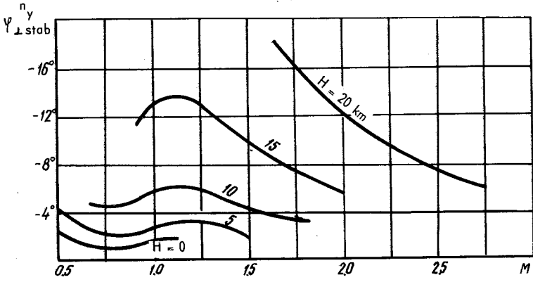
FIG. 26. DIAGRAM OF STABILIZER DEFLECTION ANGLES \psi_{\Delta \text{stab}}^{n_y} REQUIRED FOR PRODUCING G-LOAD OF 1G VERSUS MACH NUMBER. AIRCRAFT CARRIES FOUR MISSILES P-40I ( \bar{X}_{C.G.} = 19\% \text{ MAC} , G = 30 \text{ tf} )
