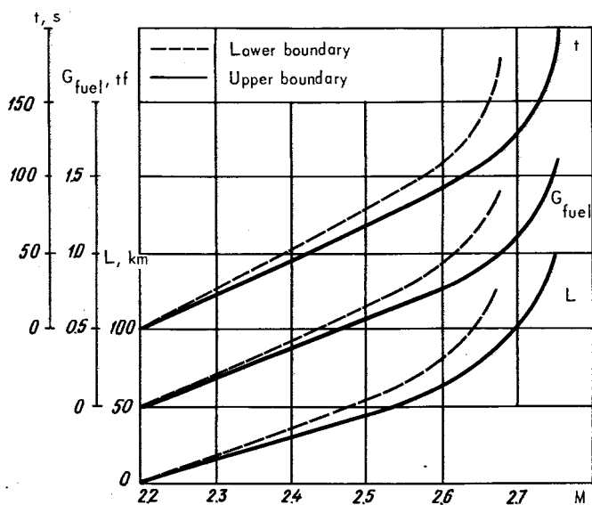
FIG. 15. ACCELERATION CHARACTERISTICS OF AIRCRAFT CARRYING FOUR MISSILES AT FULL REHEAT POWER SETTING ( H = 18,000 m, G = 25 tf, n_{en} = 100\% )
