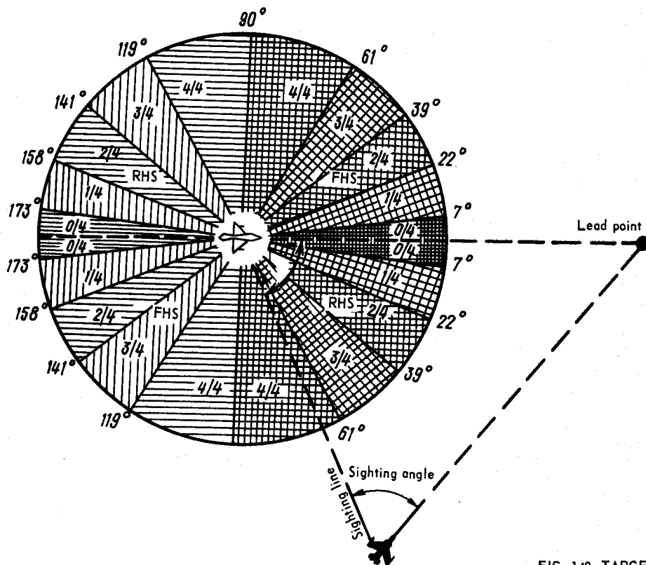
FIG. 149. TARGET ASPECT ANGLE DETERMINATION PATTERN
