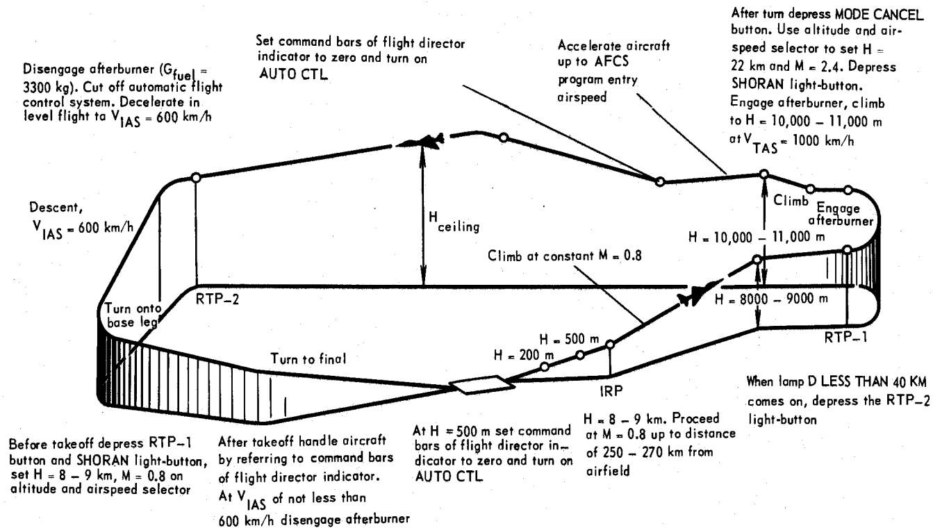
FIG. 43. FLIGHT TO SERVICE CEILING WITH USE OF AUTOMATIC MODE OF CAY-155ПДБ AUTOMATIC FLIGHT CONTROL SYSTEM
