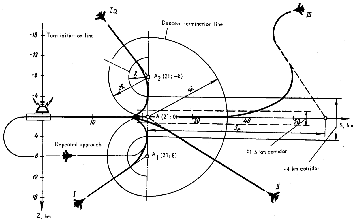
FIG. 65. INTERCEPTION OF LANDING COURSE BY AIRCRAFT IN HORIZONTAL PLANE
