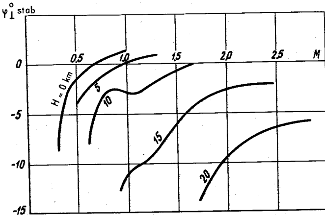
FIG. 23. DIAGRAM OF STABILIZER DEFLECTION ANGLES \psi_{st} REQUIRED FOR STRAIGHT-AND-LEVEL FLIGHT VERSUS MACH NUMBER. AIRCRAFT CARRIES FOUR MISSILES P-40Д ( \bar{x}_{C.G.} = 19\% MAC, G = 30 tf)
