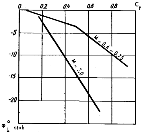
FIG. 22. STABILIZER DEFLECTION TRIMMING DEPENDENCE ON LIFT COEFFICIENT. AIRCRAFT CARRIES FOUR MISSILES P-40.1 ( \bar{X}_{\text{C.G.}} = 19\% \text{ MAC}, G = 30 \text{ tf} )
