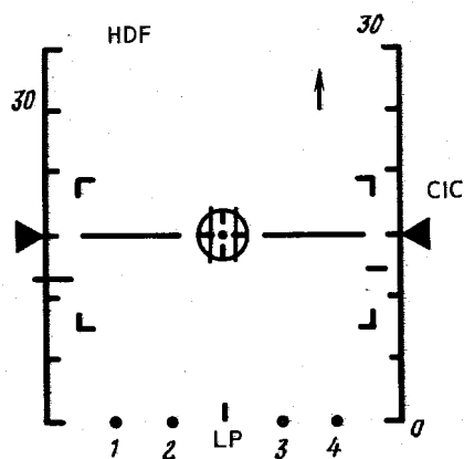
FIG. 136. PICTURE DISPLAYED ON RADAR INDICATOR SCREEN IN VISUAL DIRECTION (mode T-I, after target lockon by heat direction finder)
