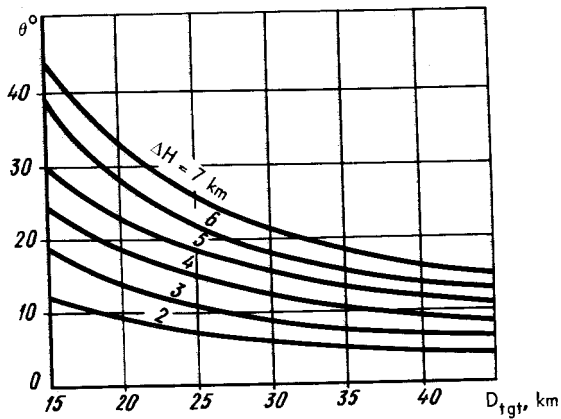
FIG. 161. ZOOM ANGLES \theta REQUIRED FOR MISSILE LAUNCHING WITH ZERO SIGHTING ERRORS IN VERTICAL PLANE VERSUS TARGET STEP-UP VERTICAL SEPARATION \Delta H AND TARGET DISTANCE D_{tgt}
