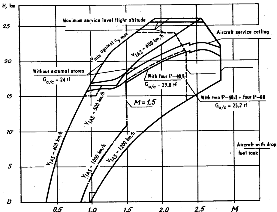
FIG. 7. ALTITUDE AND AIRSPEED RANGES OF AIRCRAFT МиГ-25ИИ
