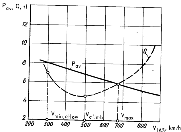
FIG. 6. CURVES OF REQUIRED AND AVAILABLE THRUSTS OF AIRCRAFT CARRYING FOUR MISSILES P-401 (non-reheat power setting, n_{en} = 80\% , H = 0 )
