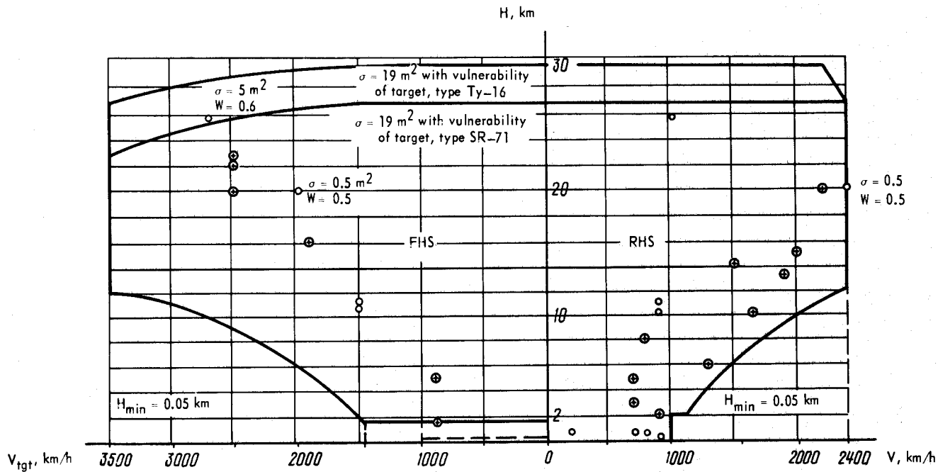
FIG. 95. RANGE OF ALTITUDES AND AIRSPEEDS OF NON-MANEUVERING TARGETS DESTROYED BY COMPLEX M_{\text{M}}^{\text{I}}-25-40.1 ( M_{\text{M}}^{\text{I}}-25-40.1\text{C} ) WITH AT LEAST 0.7 PROBABILITY WITHOUT ACCOUNTING FOR RELIABILITY
