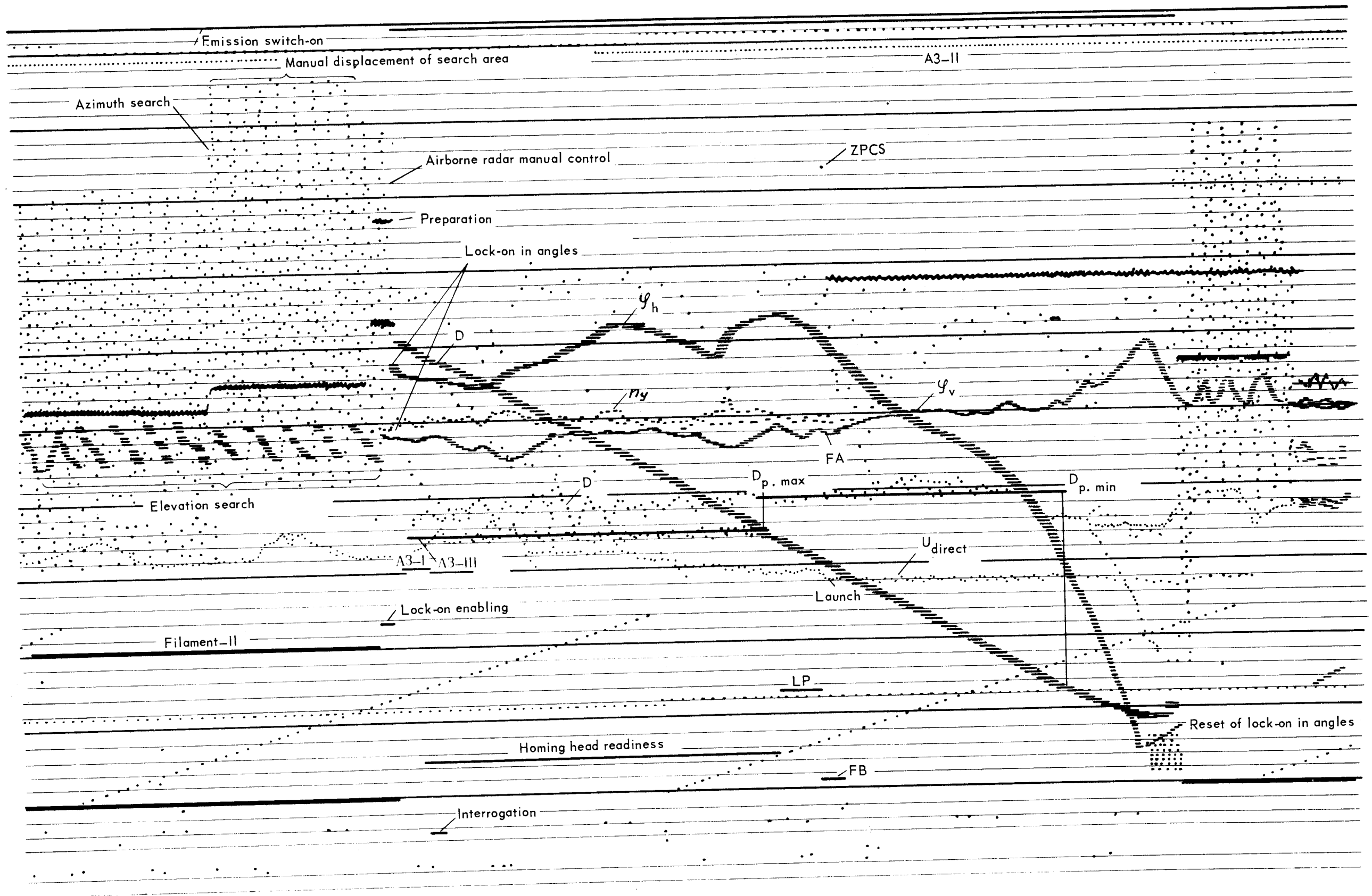
FIG. 174. EXAMPLE OF COMBAT EMPLOYMENT SIGNAL RECORD
