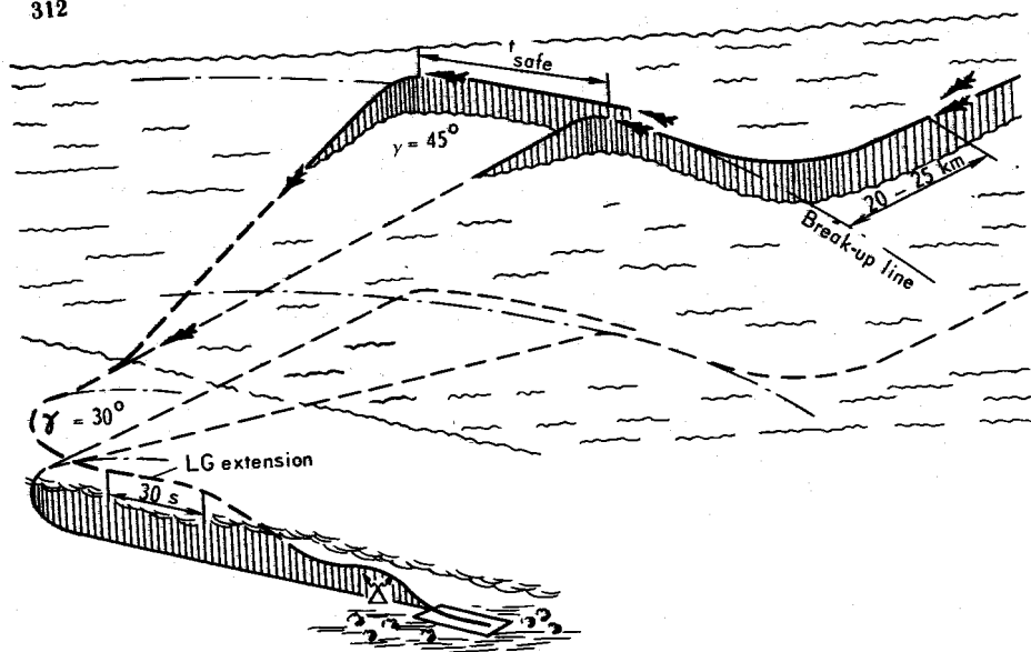
FIG. 89. PAIR BREAK-UP ON DESCENT LINE FOR DOWNWARD CLOUD PENETRATION TO HIT ESTIMATED POINT
