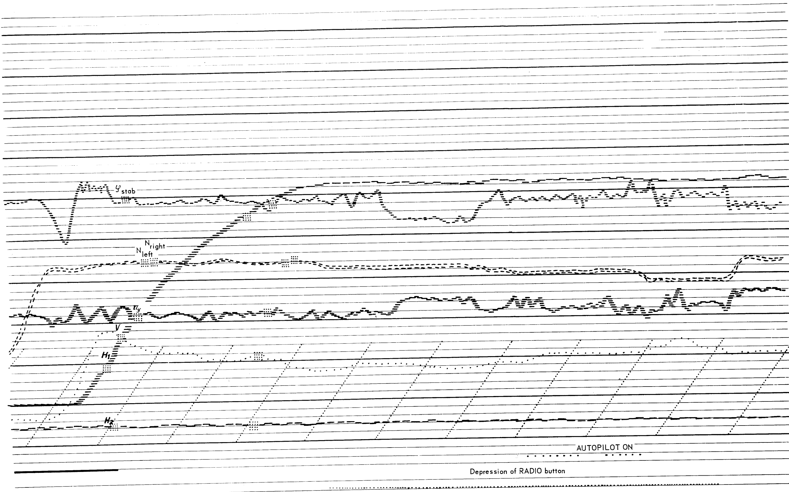
FIG. 168. EXAMPLE OF TAKEOFF SIGNAL RECORD
