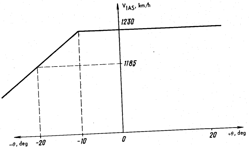
FIG. 37. PROGRAM FOR COMPUTATION OF LIMITATION OF MAXIMUM INDICATED AIRSPEED
