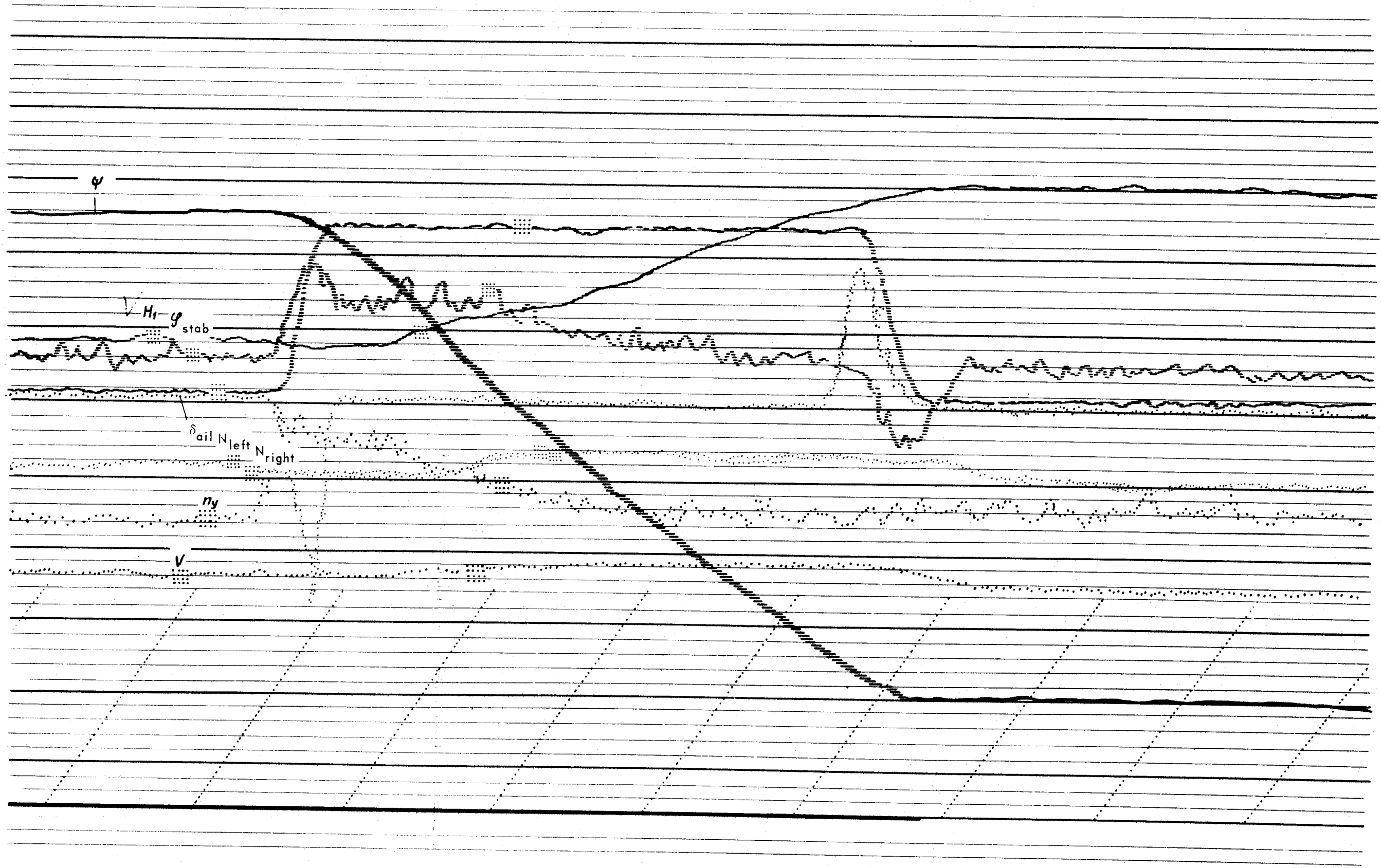
FIG. 171. EXAMPLE OF CHANDELLE SIGNAL RECORD
