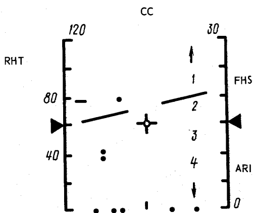
FIG. 104. PICTURE DISPLAYED ON RADAR INDICATOR SCREEN IN AUTOMATIC DIRECTION (illumination ON, modes HMA and HMA-ΔH, INTERROG button is depressed)
