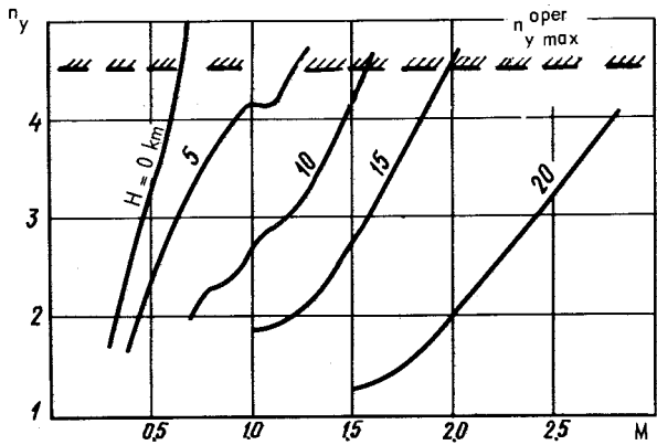
FIG. 10. AVAILABLE G-LOADS OF AIRCRAFT VERSUS MACH NUMBER AND ALTITUDE OF FLIGHT ( G = 30 \text{ ft} )
