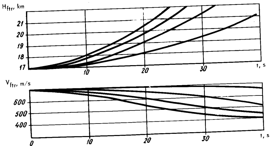
FIG. 162. VARIATION OF FIGHTER ALTITUDE AND AIRSPEED WHEN PERFORMING PREPARATORY ZOOM AT VARIOUS VERTICAL G-LOADS ( H_{ref} = 17 \text{ km} , M = 2.35 , G = 28.5 t , \gamma = 0^\circ )
