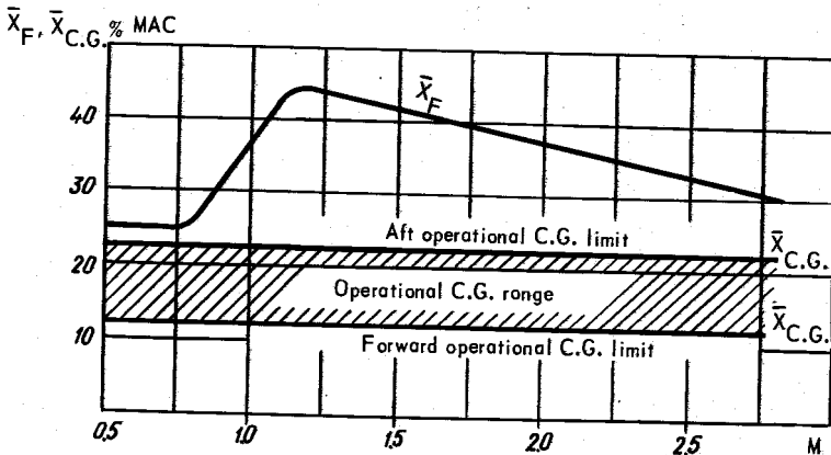
FIG. 20. DISPLACEMENT OF GROSS AERODYNAMIC CENTER X_F VERSUS MACH NUMBER OF FLIGHT (the aircraft carries four missiles P-40\Pi, with engines running)
