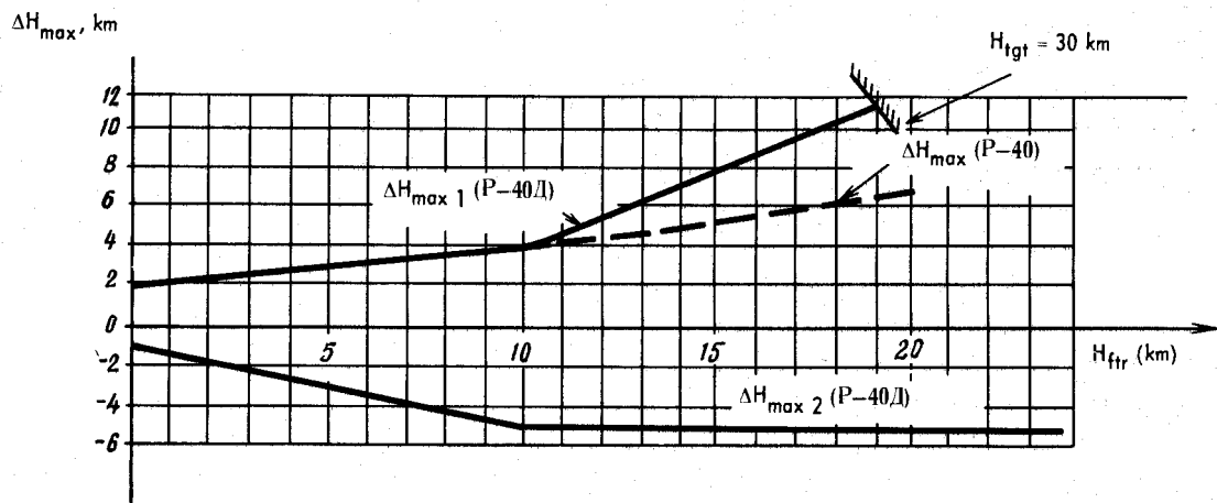
FIG. 96. PERMISSIBLE STEPPED-UP (STEPPED-DOWN) VERTICAL SEPARATIONS OF TARGET RELATIVE TO FIGHTER ALTITUDE IN LAUNCHING OF MISSILES P-40I
