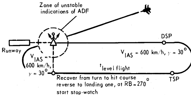
FIG. 76. 180-DEGREE TURN LANDING APPROACH PATTERN
