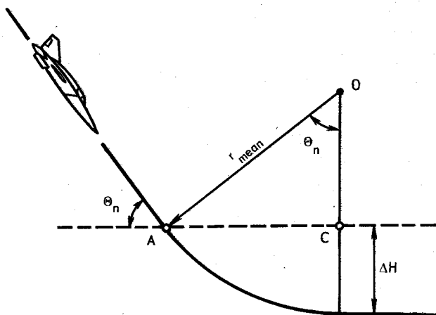
FIG. 18. DETERMINING LOSS OF ALTITUDE \Delta H DURING RECOVERY FROM DIVE
