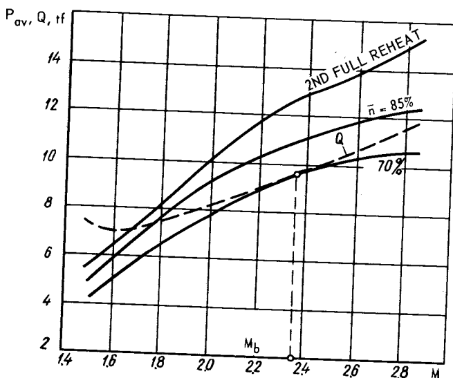
FIG. 5. CURVES OF REQUIRED AND AVAILABLE THRUSTS OF AIRCRAFT CARRYING FOUR MISSILES P-401 AT REHEAT POWER SETTING ( H = 18,000 m)
