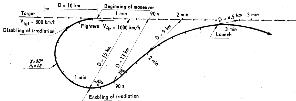
FIG. 157. PATTERN OF MANEUVER PERFORMED BY PAIR OF FIGHTERS
