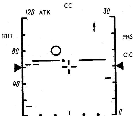
FIG. 113. PICTURE DISPLAYED ON RADAR INDICATOR SCREEN AT HOMING STAGE (missile P-40.1, fighter position control, mode HMA)
