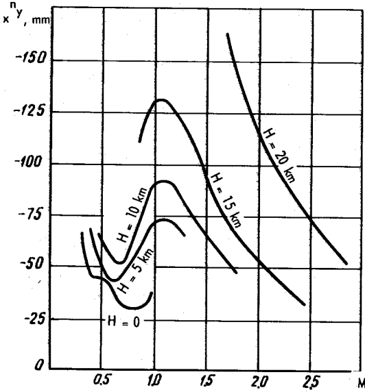
FIG. 24. DIAGRAM OF STICK TRAVEL x^ny REQUIRED FOR PRODUCING G-LOAD OF 1G VERSUS MACH NUMBER. AIRCRAFT CARRIES FOUR MISSILES P-40I ( \bar{x}_{C.G.} = 19\% MAC, G = 30 \text{ tf} )
