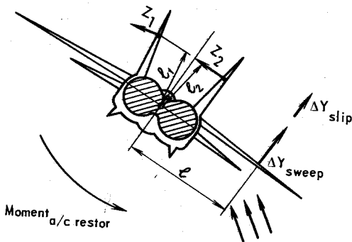
FIG. 30. FORCES AND MOMENTS ACTING UPON AIRCRAFT WHEN EQUILIBRIUM ABOUT ROLLING AXIS IS DISTURBED
