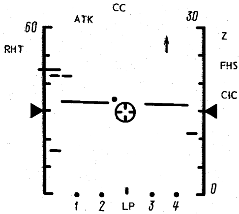
FIG. 114. PICTURE DISPLAYED ON RADAR INDICATOR SCREEN IN HOMING STAGE (missile P-401, fighter position control, mode HMA, launch permitted)
