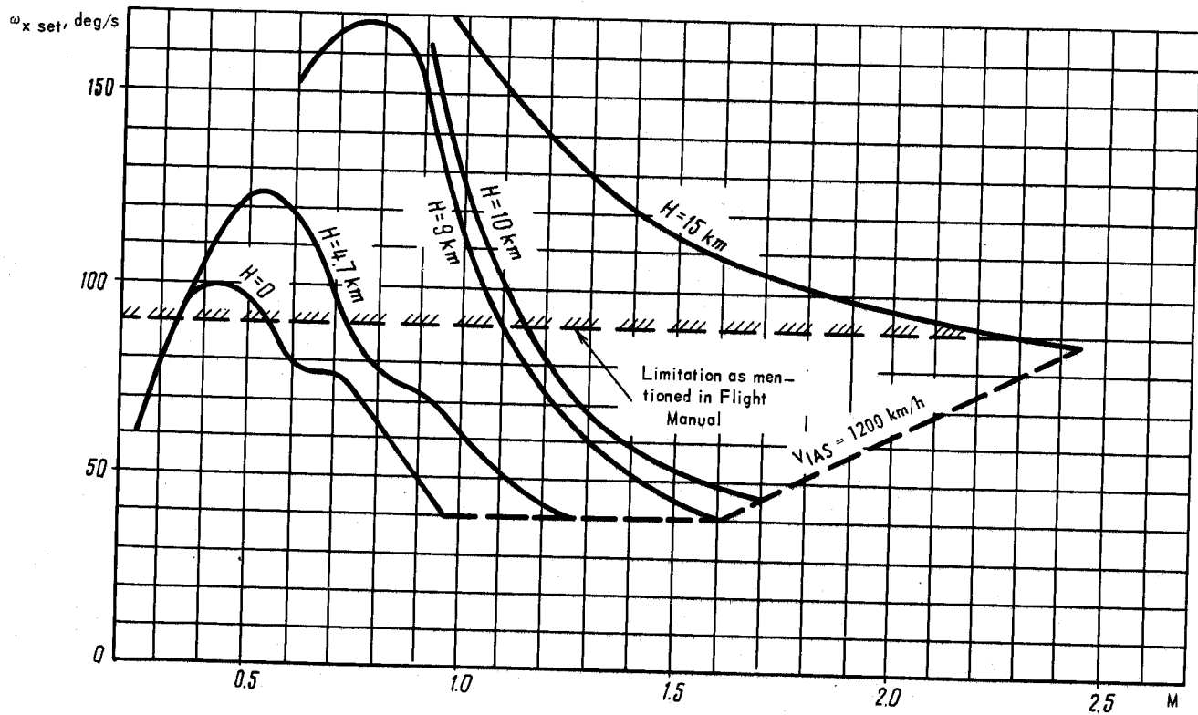
FIG. 32. MAXIMUM AVAILABLE AIRCRAFT RATE OF ROLL
