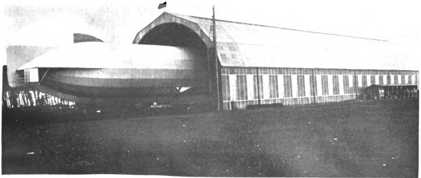
AIRSHIP SHED AT FRANKFORT-ON-THE-MAIN (GERMANY)
