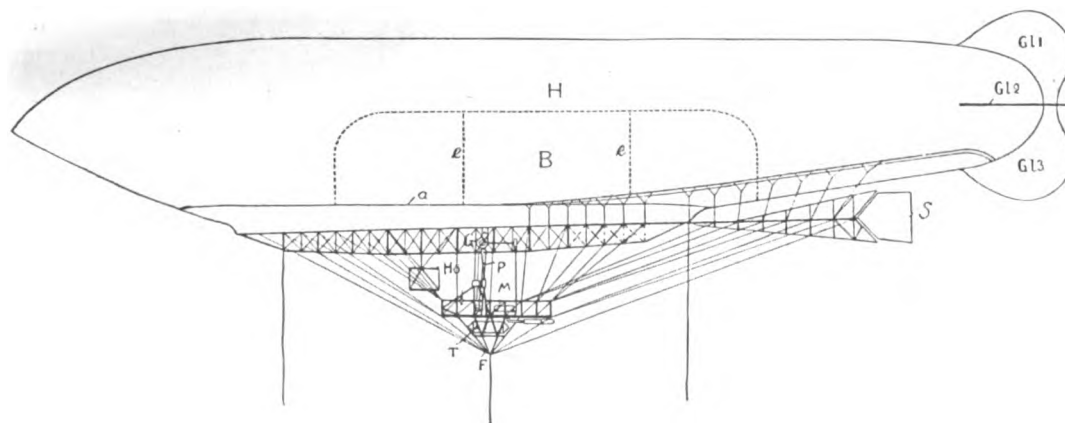
DIAGRAM OF THE 7,000 CBM. LEBAUDY AIRSHIP CAPITAINE-MARCHAL (KEEL-GIRDER, PRESSURE TYPE).
