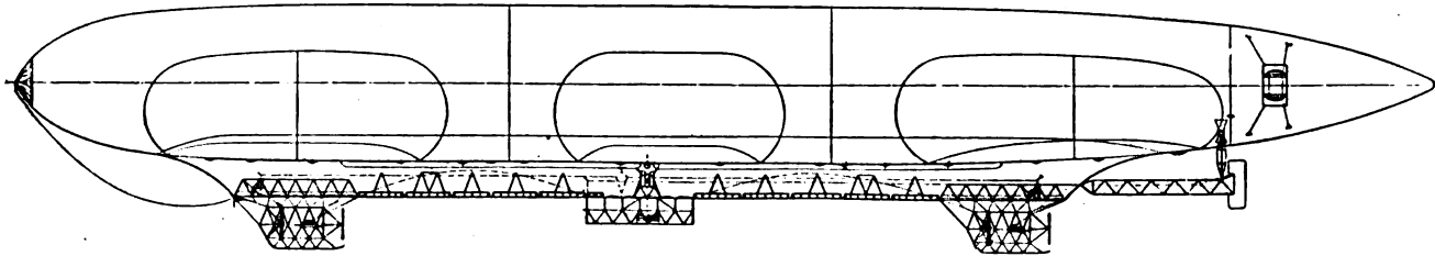
DIAGRAM OF THE 13,000 CBM. SIEMENS-SCHUCKERT AIRSHIP S. S. 1 (GIRDERLESS PRESSURE TYPE; RIGGING BAND REINFORCED BY A FLEXIBLE KEEL OF FABRIC STRIPS).
