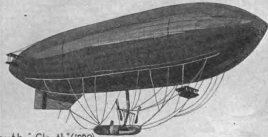
Clouth - "Clouth" (1909)
