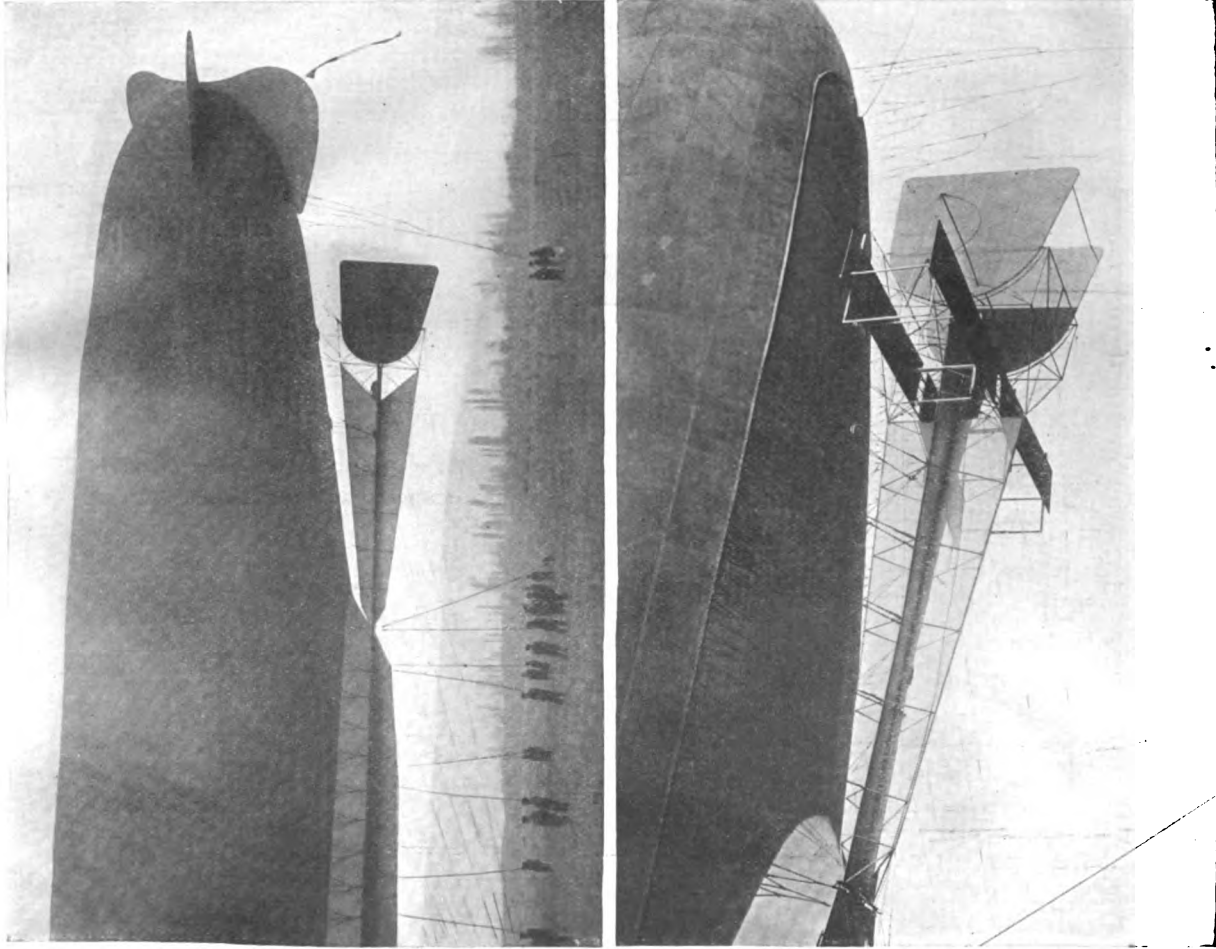
STERN VIEW OF THE LIBERTÉ AND OF THE CAPITAINE-MARCHAL.
