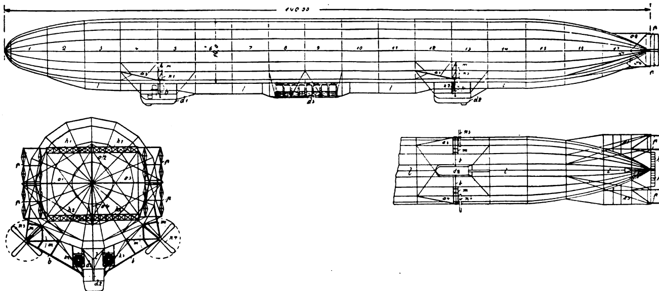
DIAGRAM OF AN 18,000 CBM. ZEPPELIN AIRSHIP, THE SCHWABEN (STRUCTURE TYPE).
