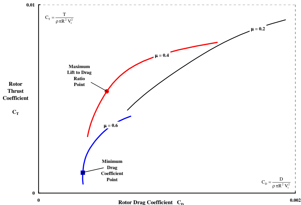
Figure 3. Typical Lift–Drag Polars for a Conventional Rotor.
