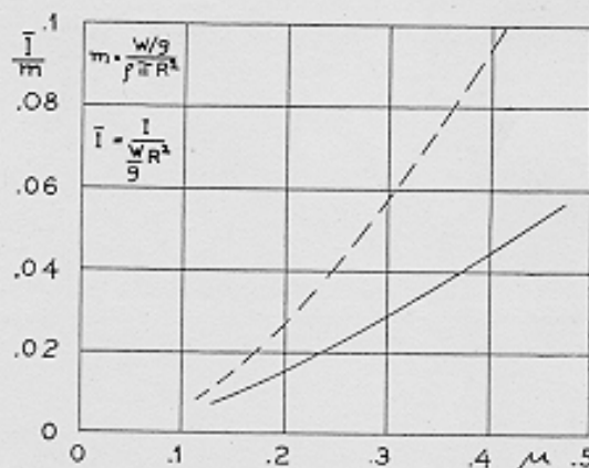
FIG. 13. Maximum allowable helicopter moment of inertia about pitching axis against \mu for dynamic stability when using sample rotor with pitch-cone change. Solid lines for constant torque; dashed lines for constant rotor speed.
