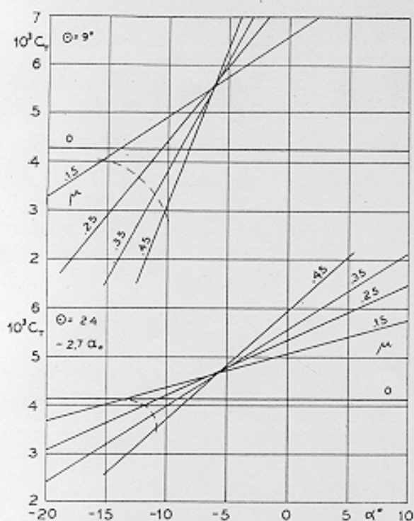
FIG. 7. Comparison between fixed-pitch rotor (above) and rotor with pitch-cone change (below). Thrust coefficient c_T against \alpha with advance ratio \mu as parameter. Dashed lines for constant c_q/c_r equal to c_q/c_r in hovering.
