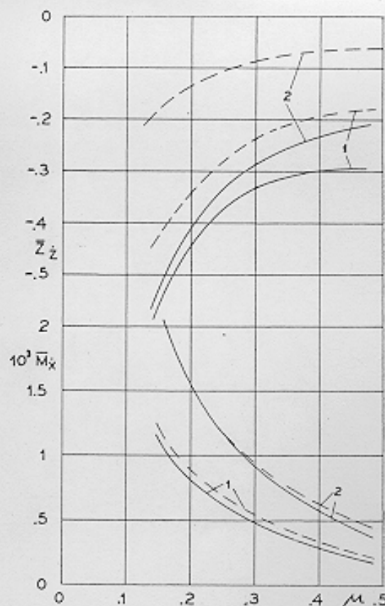
FIG. 11. Vertical damping -Z_z and velocity stability M_x against advance ratio \mu for constant c_Q/c_T equal to c_Q/c_T in hovering. 1 for fixed pitch, \theta = 9^\circ ; 2 for sample rotor with pitch-cone change, \theta = 24 - 2.7\alpha . Solid curves for constant torque; dashed curves for constant rotor speed.
