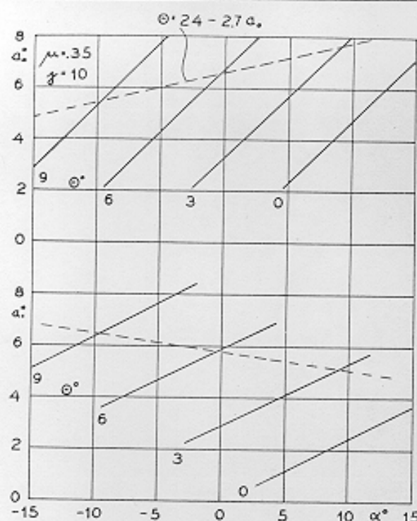
Fig. 3. Coning angle a_1 and tip path plane inclination a_2 against \alpha with blade pitch angle \theta as parameter for advance ratio \mu = 0.35 . Dashed lines for sample rotor with pitch-cone change.
