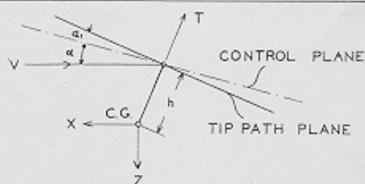
FIG. 1. Schematic side view of lifting rotor.
