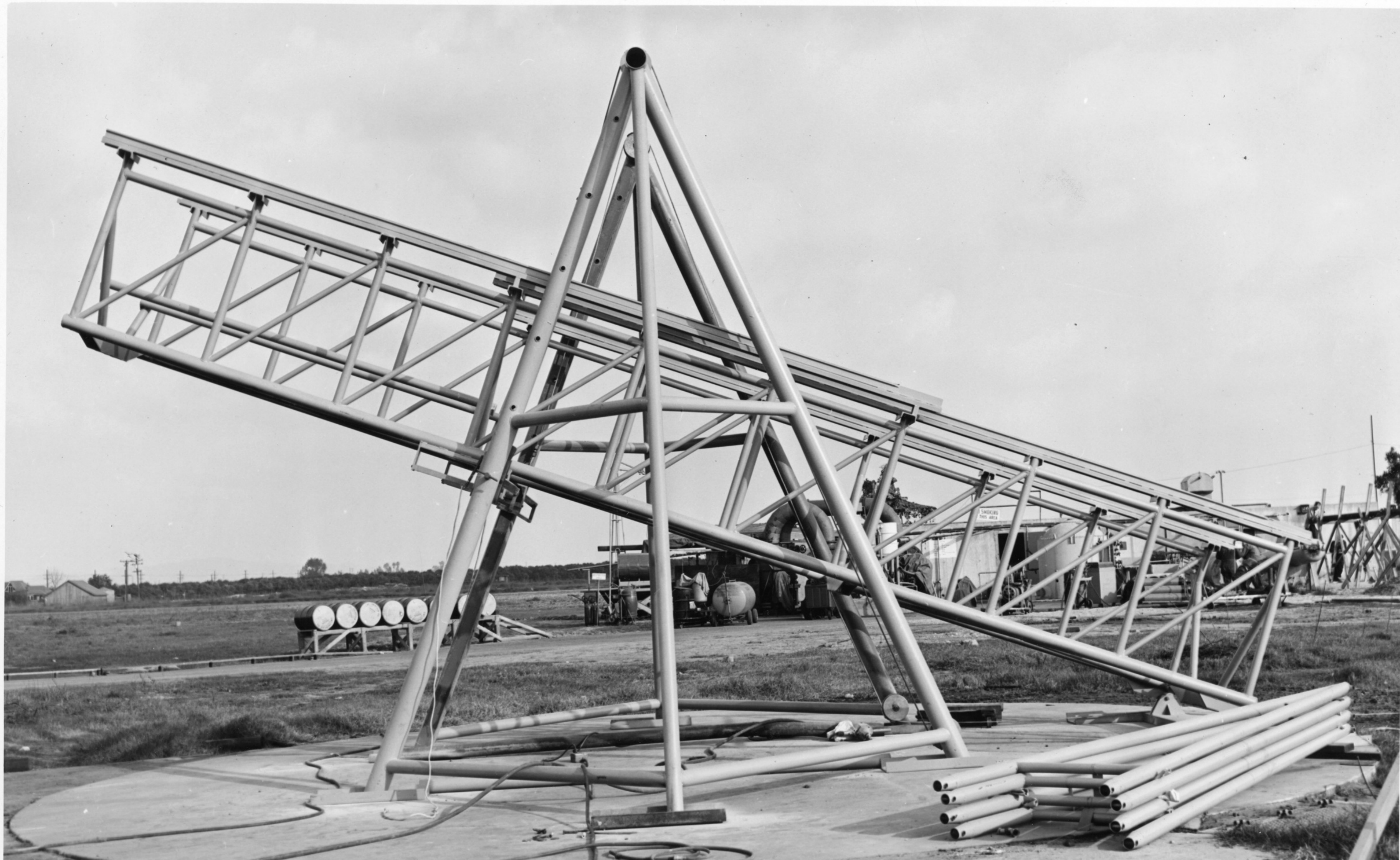
KAY-1 LAUNCHING RAMP FOR LAUNCHING AIRCRAFT WITH TWO 11000 LB ROCKETS
