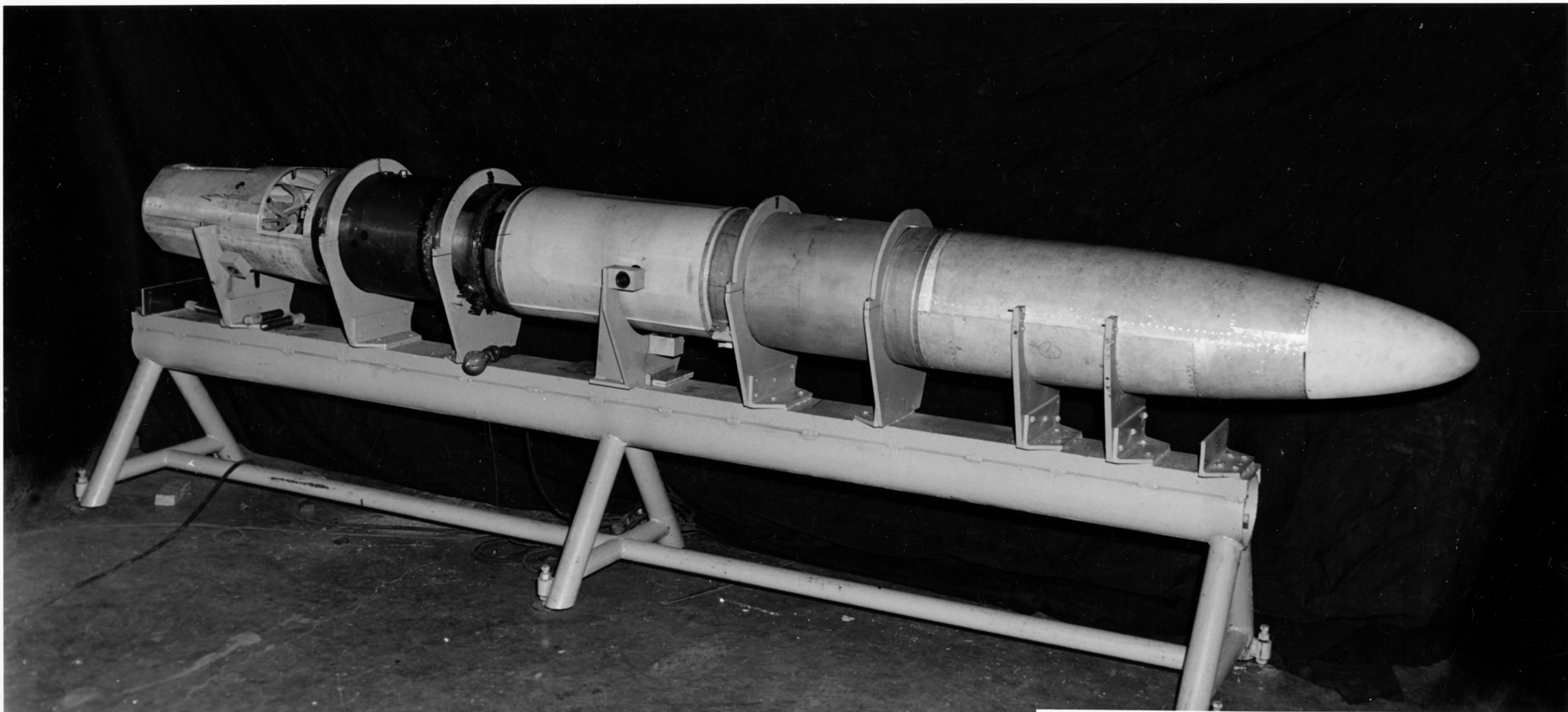
LARK NO. 1 IN ASSEM. JIG
