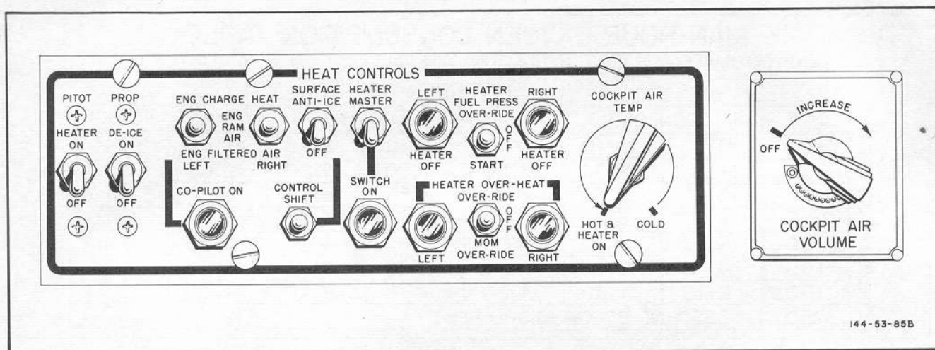
Figure 4-3. Heat Controls
