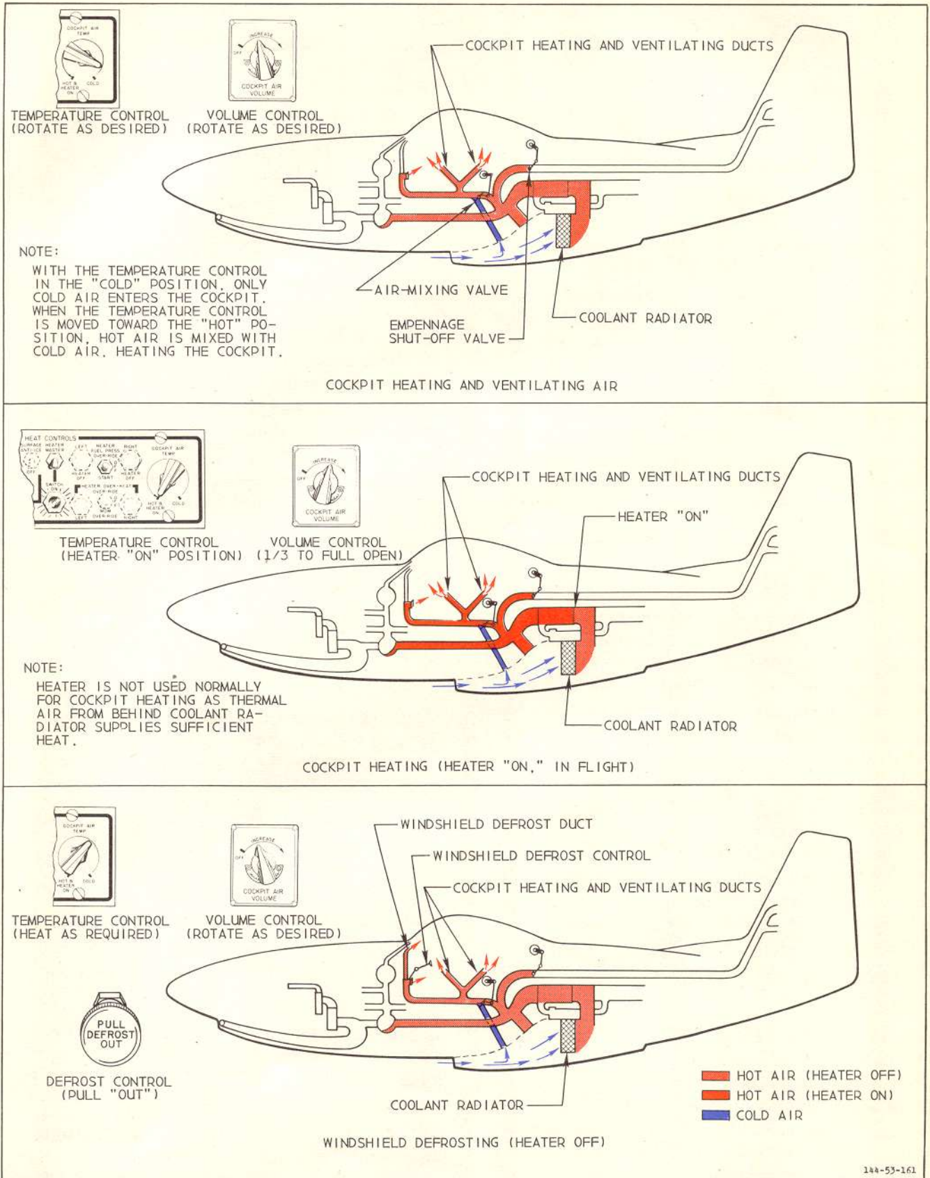
Figure 4-4. Cockpit Heating, Ventilating, and Defrosting
