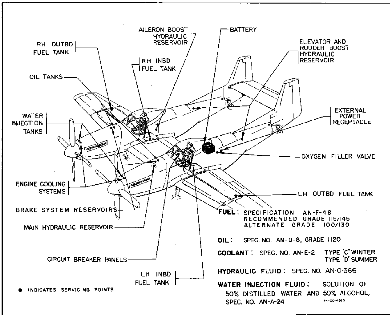
Figure 1-13. General Arrangement
