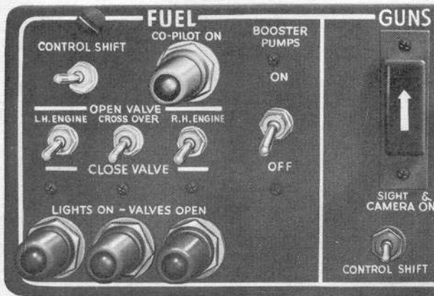
Figure 2-3. Copilot's Fuel Control Panel
