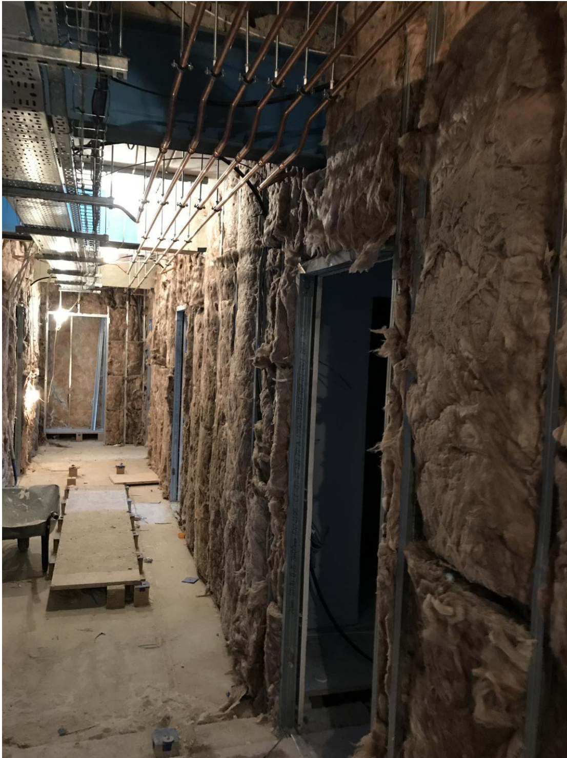
Fourth floor corridor, full M&E first fix, party wall insulation, ready for boarding
