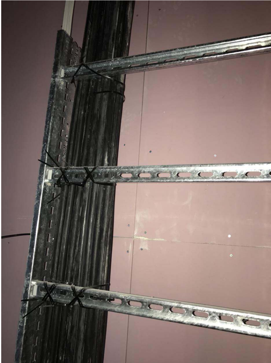
Second floor apartment submains riser
