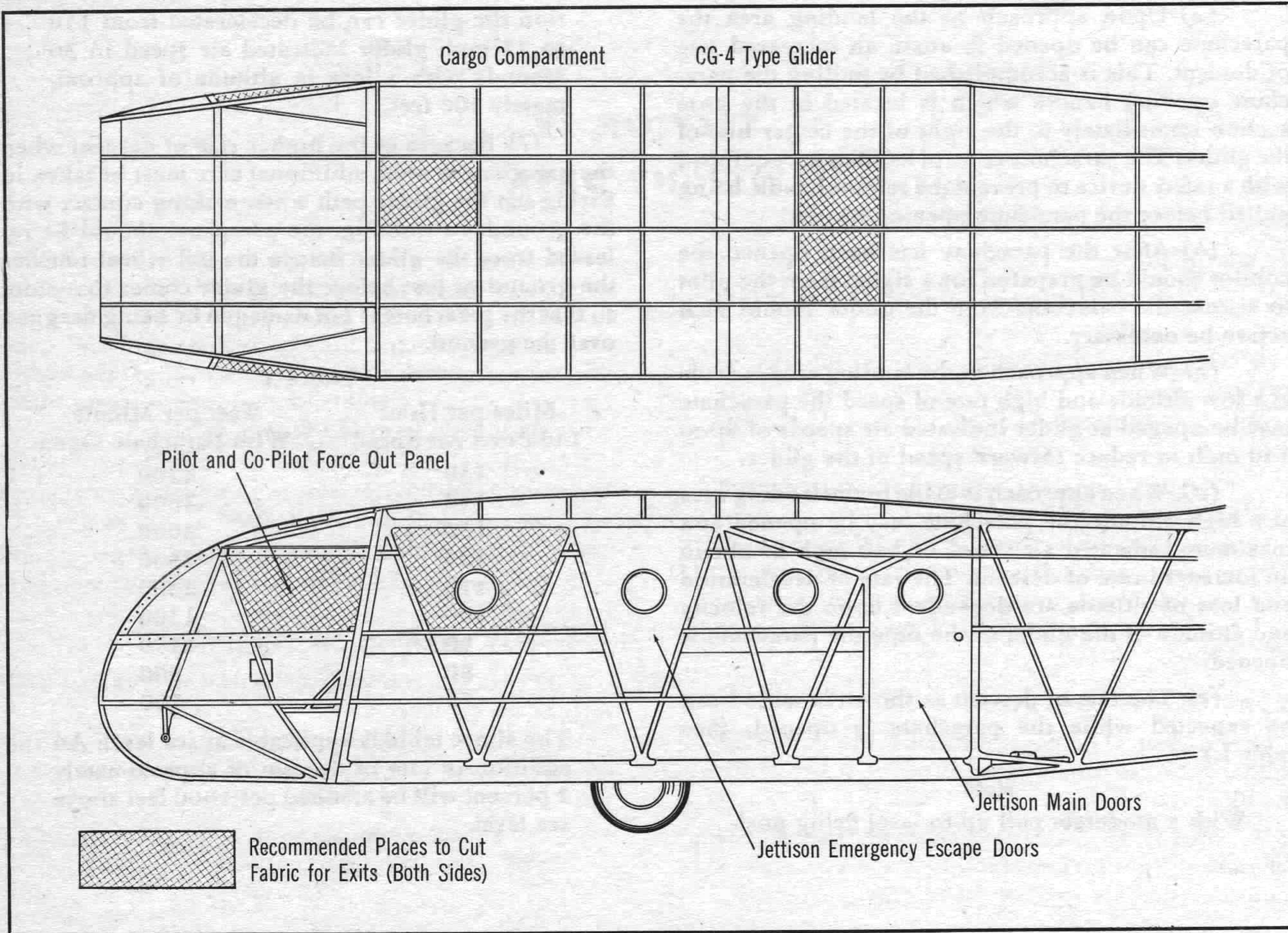
Figure 6—Emergency Exits
