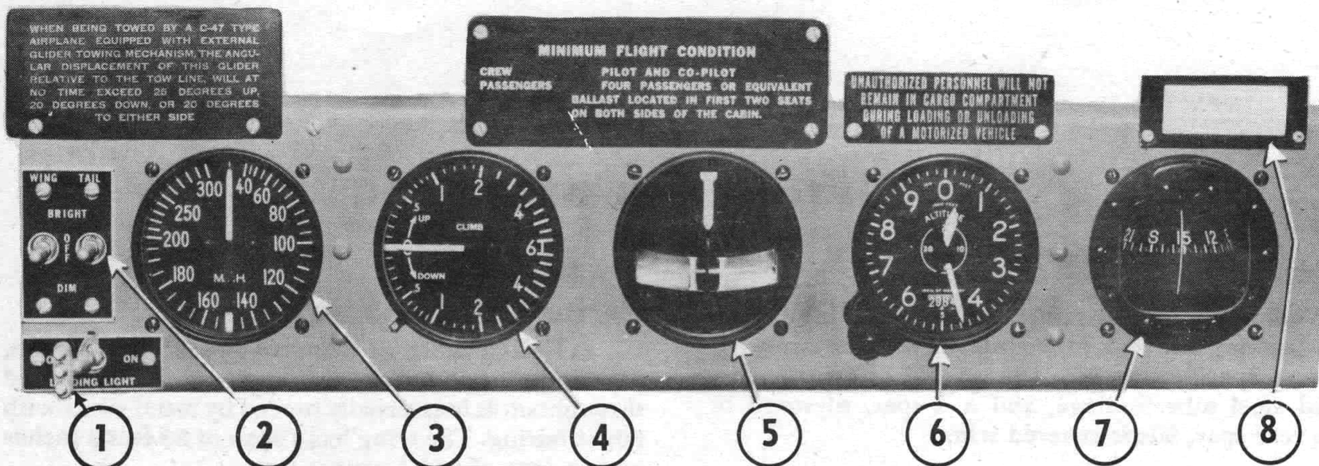
Figure 3—Instrument Panel
