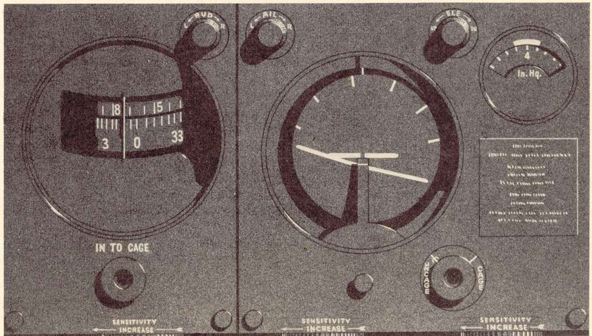
Panel of Automatic Pilot
