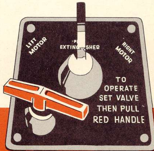
FIRE EXTINGUISHER CONTROL
