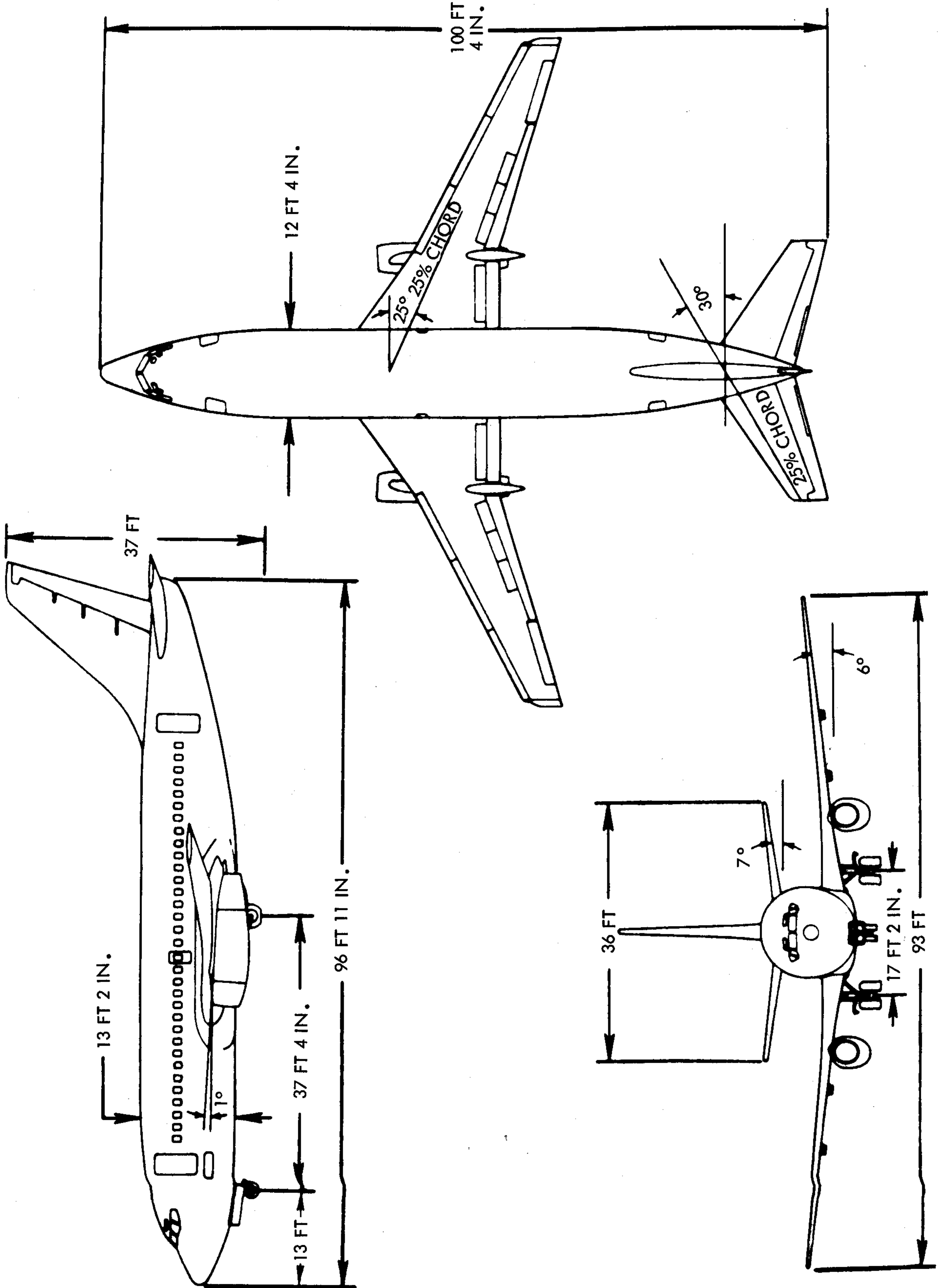
Figure 1. Principal Dimensions
