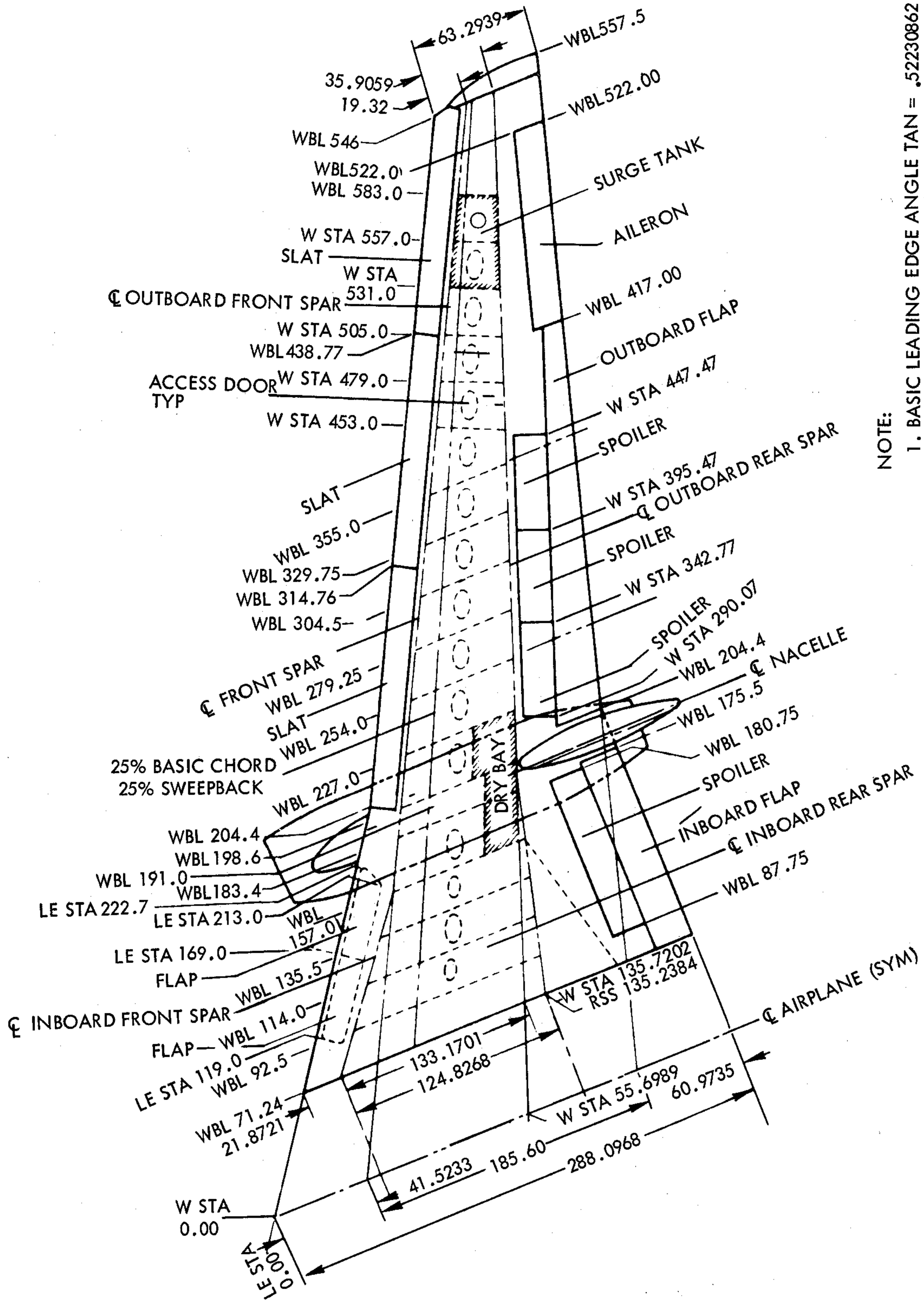
Figure 3. Wing Station Diagram
