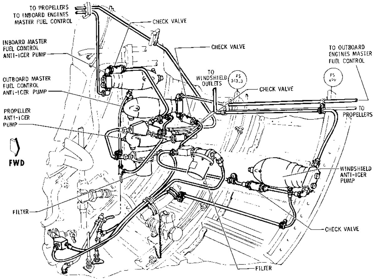
INSTALLATION OF MASTER CONTROL PROPELLER AND WINDSHIELD ANTI-ICER PUMPS
