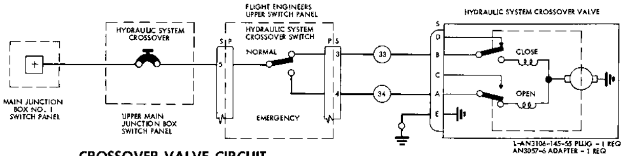
CROSSOVER VALVE CIRCUIT
