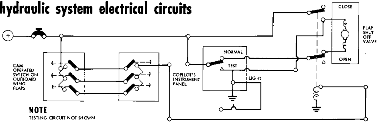
WING FLAP ASYMMETRY PROTECTION SYSTEM CIRCUIT
