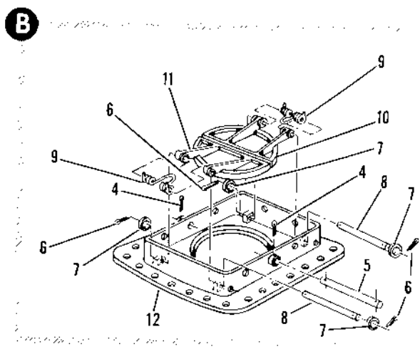
Figure 2.13-21. Armament Bay Ground Air-Conditioning Duct Installation
