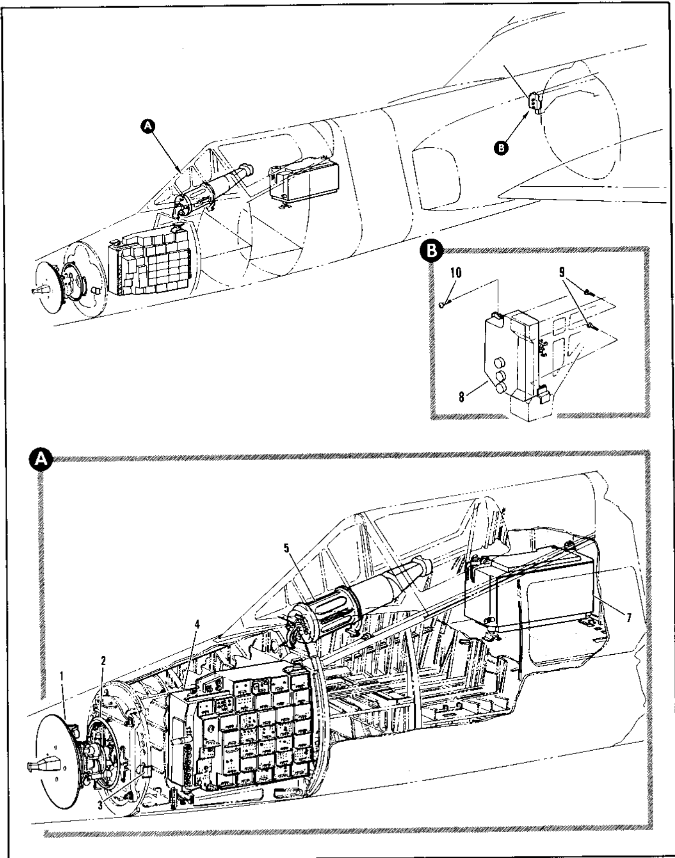
Figure 2.18-10. Radar
