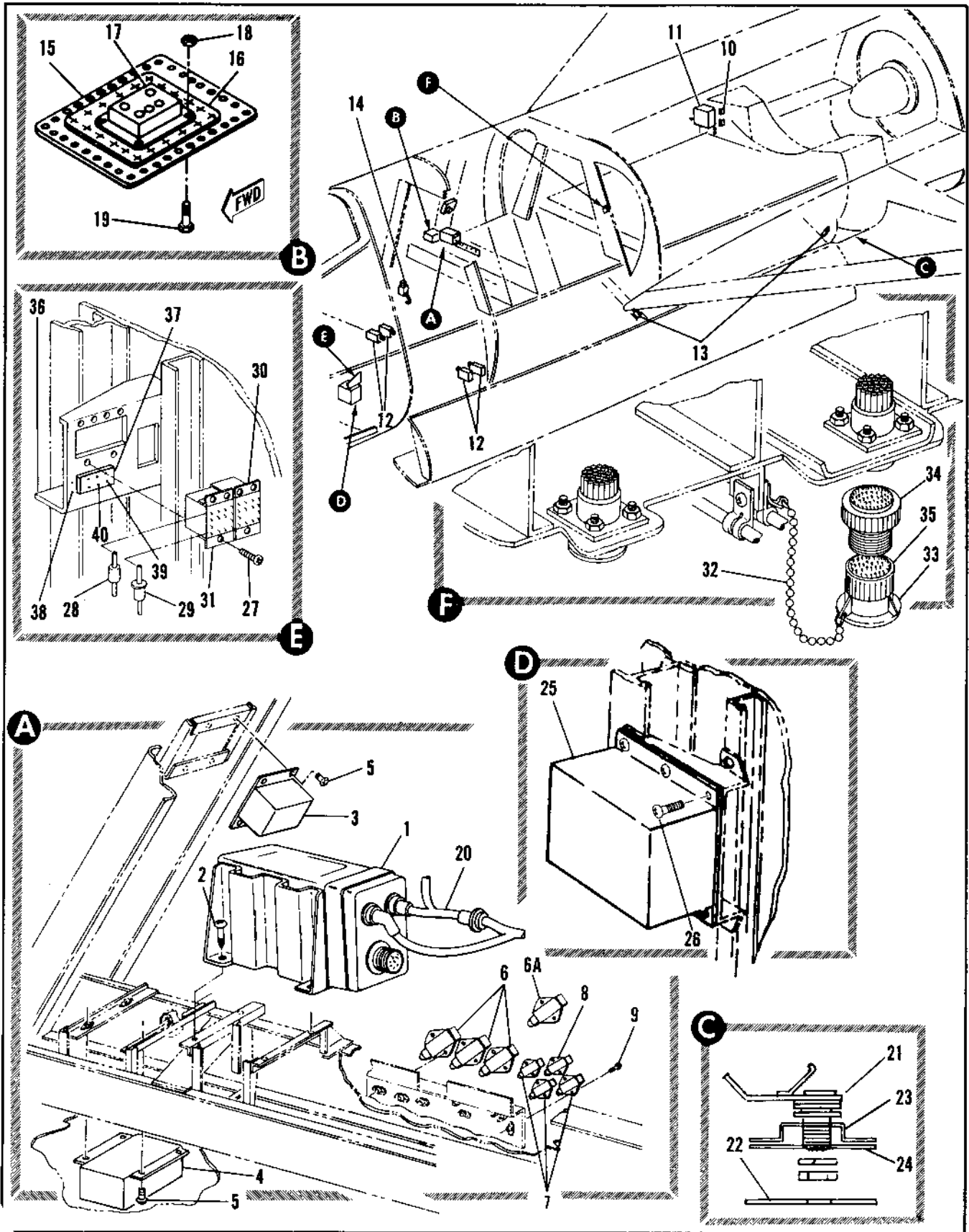
Figure 2.20-2. Armament Electrical
