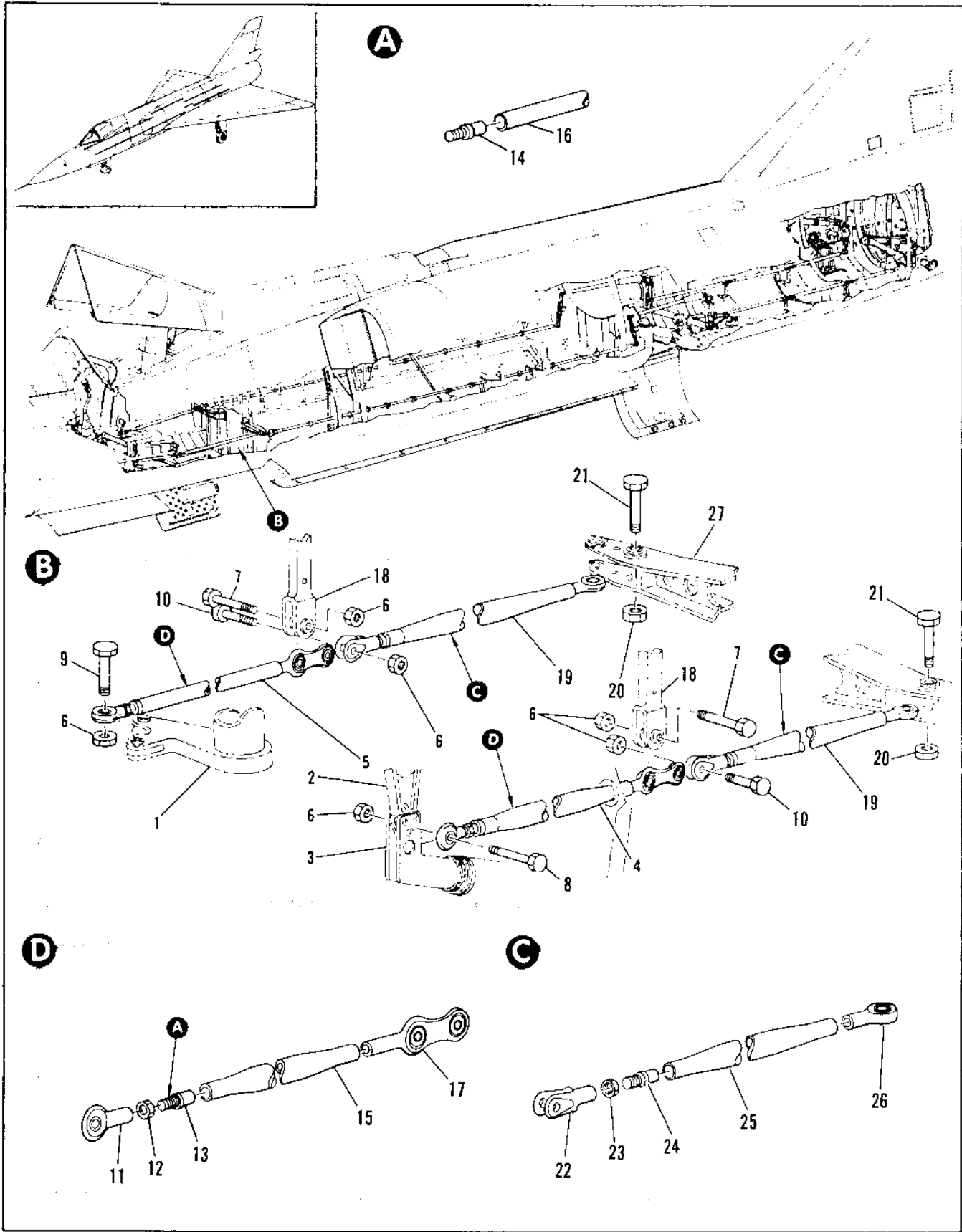
Figure 2.14-15. Elevon Control Linkage Installation (Sheet 1 of 5)
